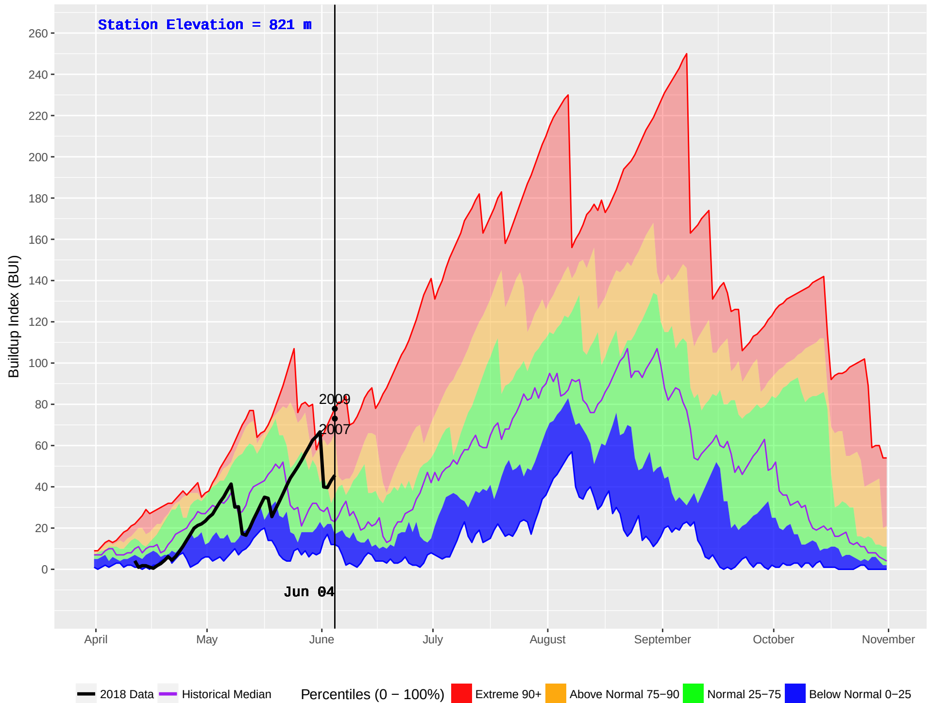
AKOKLI CREEK (838) : Historical (2003–2016) and Current (2018) Noon Buildup Index (BUI)
