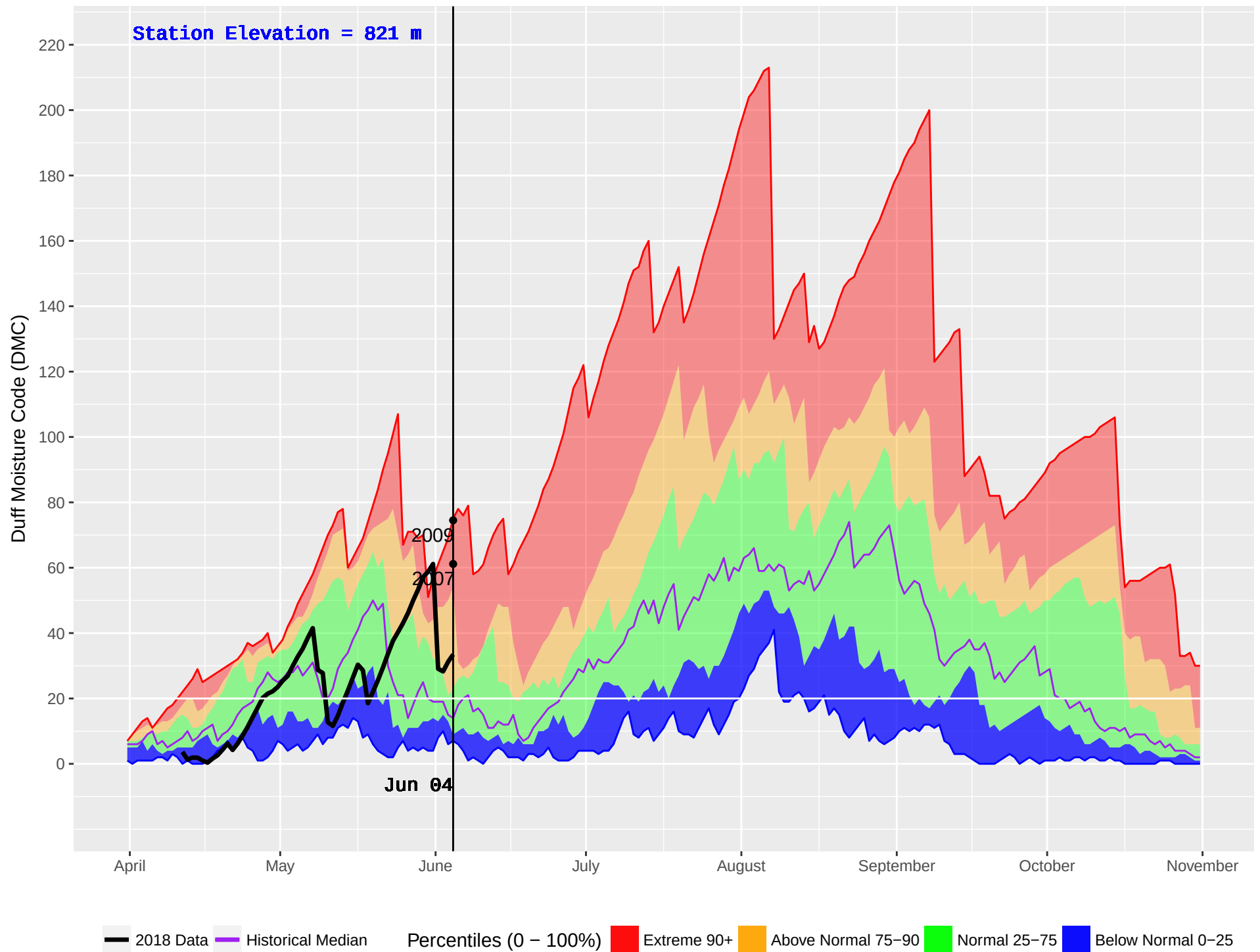
AKOKLI CREEK (838) : Historical (2003–2016) and Current (2018) Noon Duff Moisture Code (DMC)
