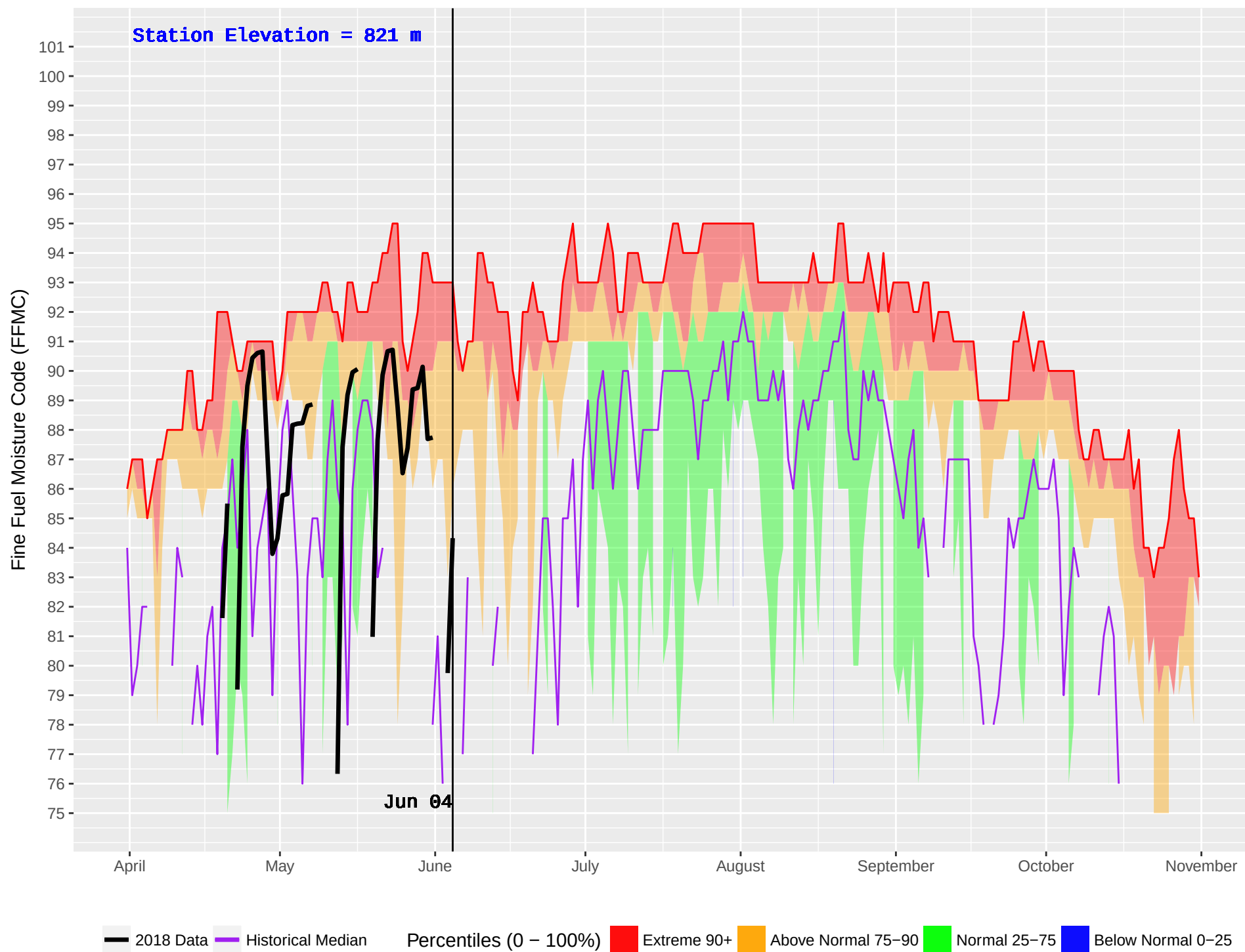
AKOKLI CREEK (838) : Historical (2003–2016) and Current (2018) Noon Fine Fuel Moisture Code (FFMC)
